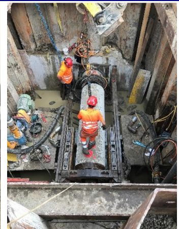
Startschacht Microtunneling
